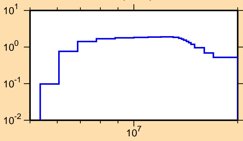
\sigma vs. E for ^{160}\text{Eu}(n,2n)
