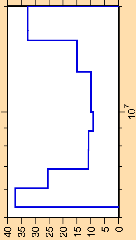
\Delta\sigma/\sigma vs. E for ^{160}\text{Eu}(n,2n)
