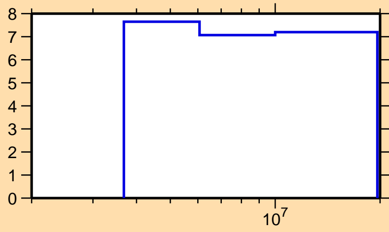
\Delta\sigma/\sigma vs. E for ^{160}\text{Eu}(n,\text{nonel.})
