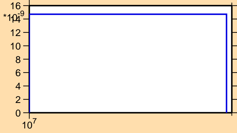
\sigma vs. E for ^{160}\text{Eu}(n,nt)
