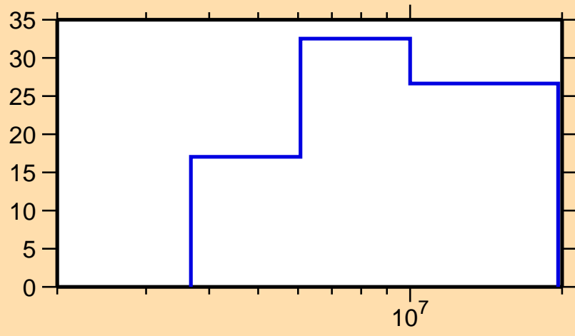
\Delta\sigma/\sigma vs. E for ^{160}\text{Eu}(n,\text{inel.})
