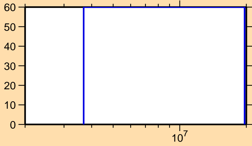
\Delta\sigma/\sigma vs. E for ^{160}\text{Eu}(n,p)
