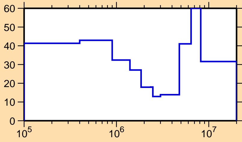
\Delta\sigma/\sigma vs. E for ^{160}\text{Eu}(n,n\text{cont.})
