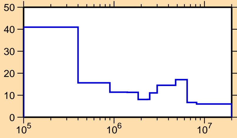
\Delta\sigma/\sigma vs. E for ^{160}\text{Eu}(n, el.)
