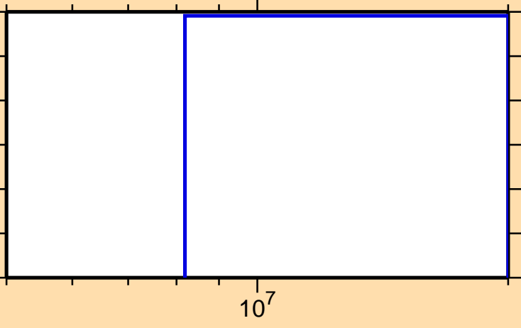
\sigma vs. E for ^{160}\text{Eu}(n,n\alpha)
