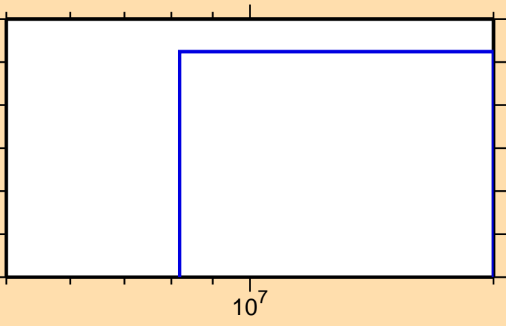
\sigma vs. E for ^{160}\text{Eu}(n,nd)
