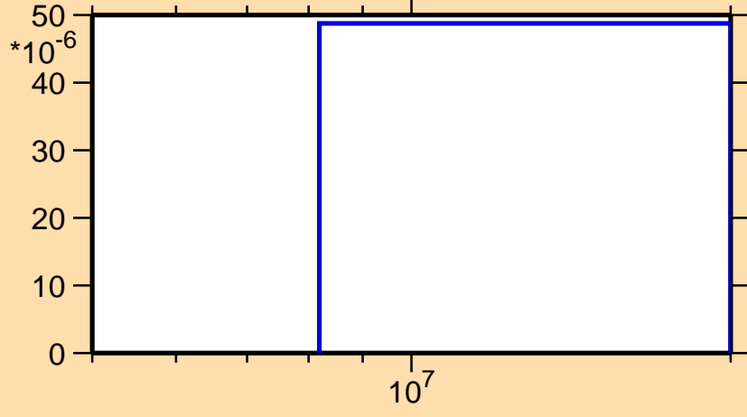
\sigma vs. E for ^{160}\text{Eu}(n,np)
