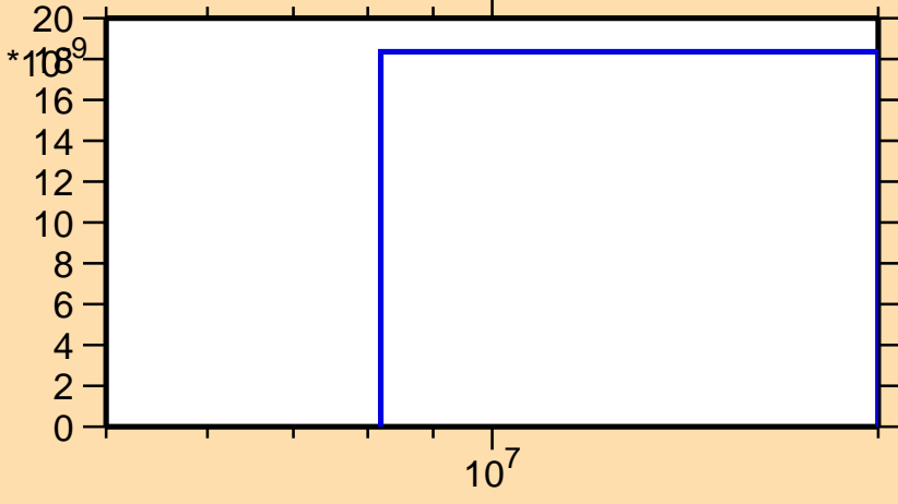
\sigma vs. E for ^{161}\text{Eu}(n,nt)
