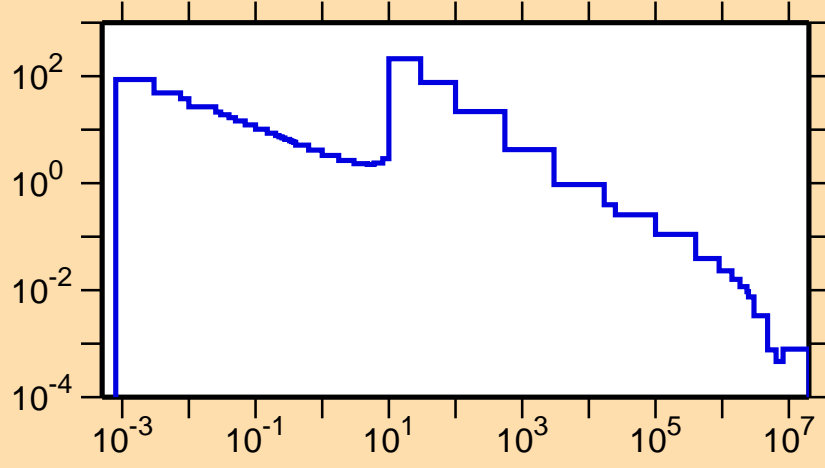
\sigma vs. E for ^{161}\text{Eu}(n,\gamma)
