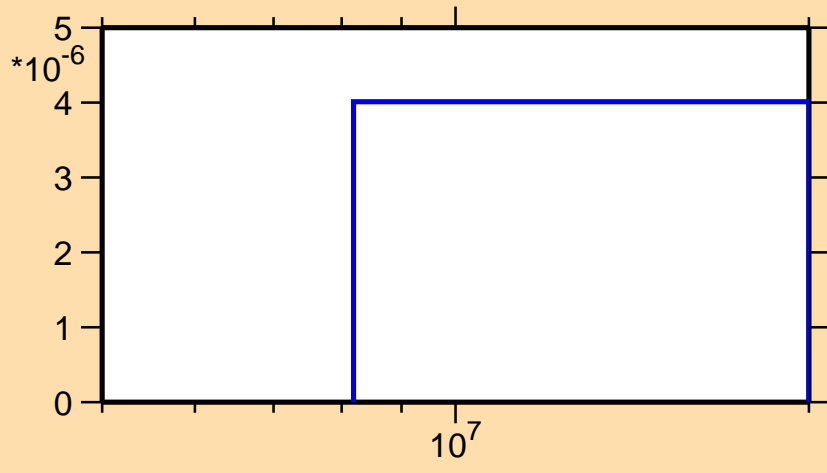
\sigma vs. E for ^{161}\text{Eu}(n,n\alpha)
