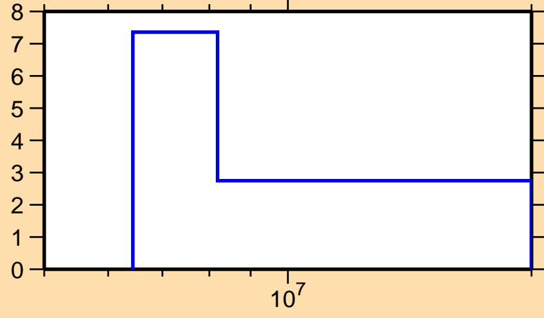
\Delta\sigma/\sigma vs. E for ^{161}\text{Eu}(n,\text{tot.})
