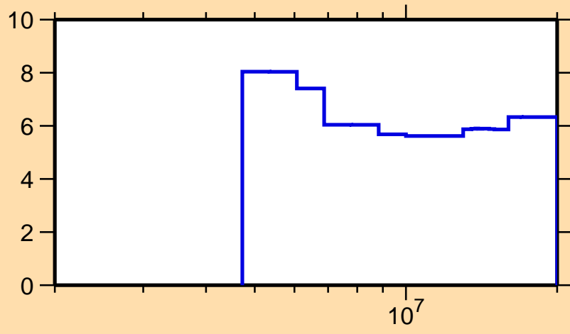
\Delta\sigma/\sigma vs. E for ^{162}\text{Eu}(n,\text{nonel.})
