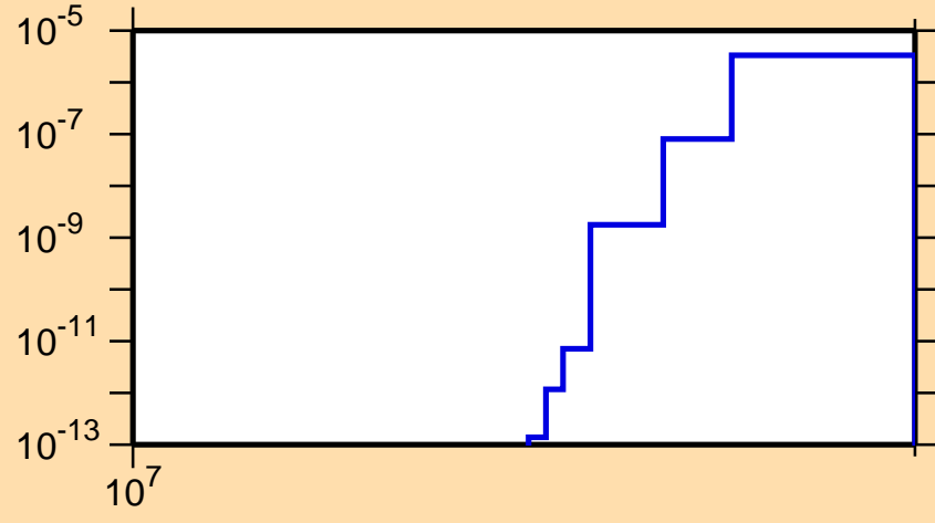
\sigma vs. E for ^{162}\text{Eu}(n,nd)
