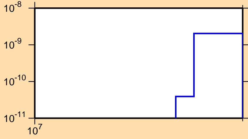
\sigma vs. E for ^{163}\text{Eu}(n,2n\alpha)
