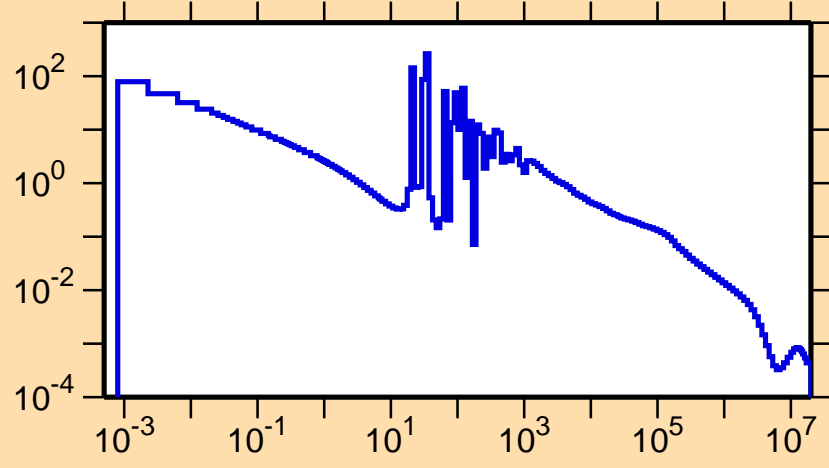
\sigma vs. E for ^{163}\text{Eu}(n,\gamma)
