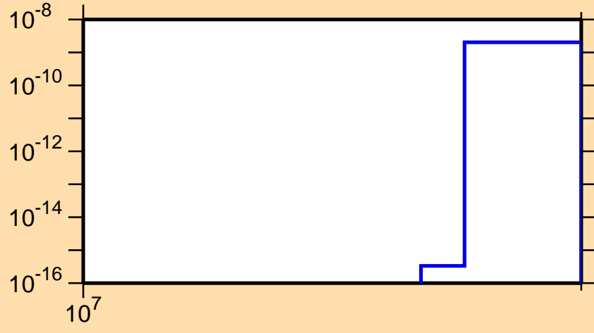
\sigma vs. E for ^{163}\text{Eu}(n,2np)
