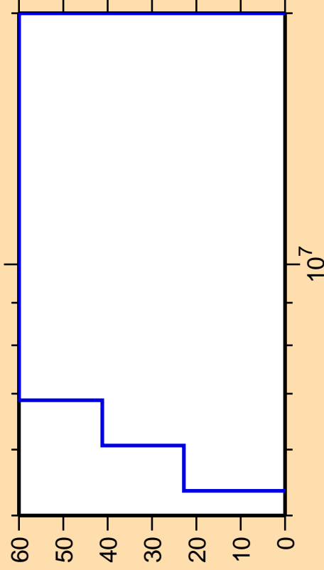
\Delta\sigma/\sigma vs. E for ^{163}\text{Eu}(n,n\text{cont.})
