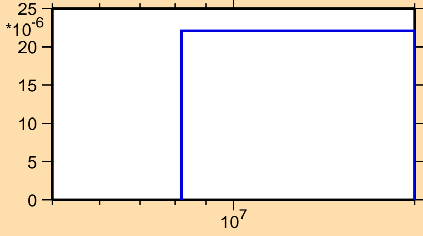
\sigma vs. E for ^{163}\text{Eu}(n,d)
