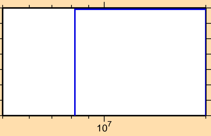
\sigma vs. E for ^{163}\text{Eu}(n,n\alpha)
