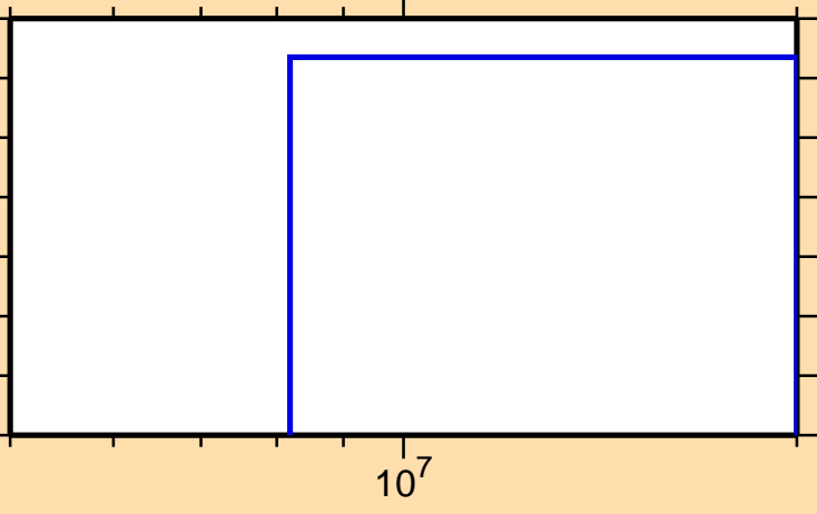
\sigma vs. E for ^{163}\text{Eu}(n,t)
