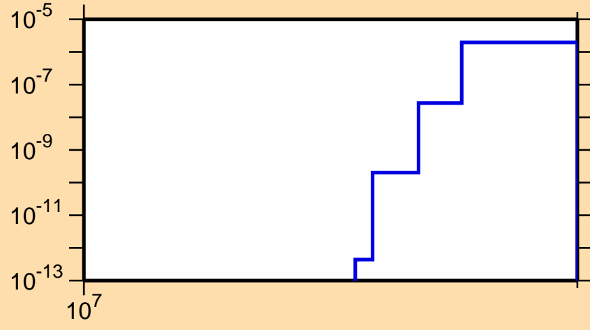
\sigma vs. E for ^{164}\text{Eu}(n,nd)
