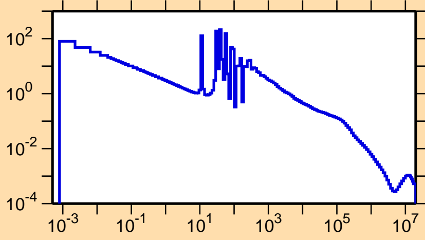
\sigma vs. E for ^{164}\text{Eu}(n,\gamma)
