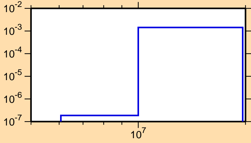
\sigma vs. E for ^{164}\text{Eu}(n,p)
