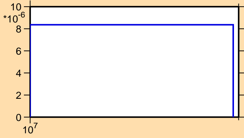
\sigma vs. E for ^{164}\text{Eu}(n,np)
