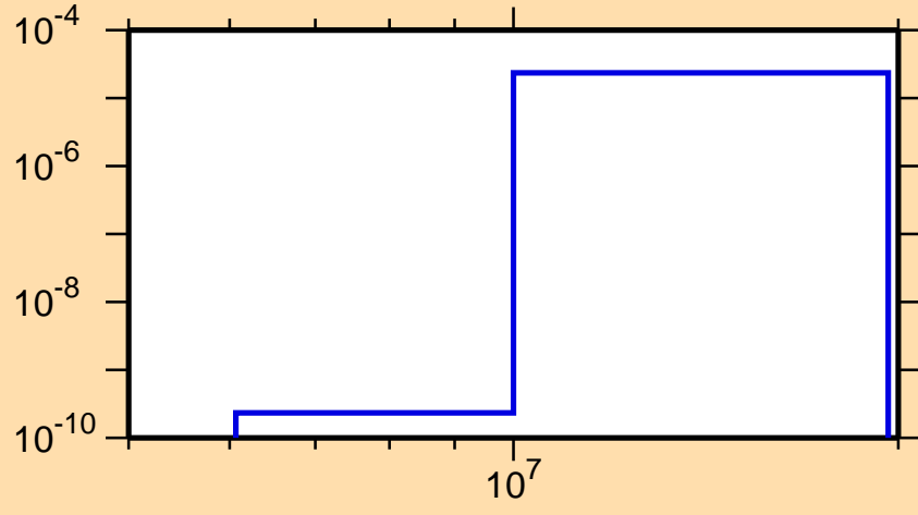
\sigma vs. E for ^{164}\text{Eu}(n,\alpha)
