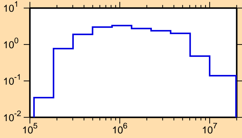
\sigma vs. E for ^{164}\text{Eu}(n,n\text{cont.})
