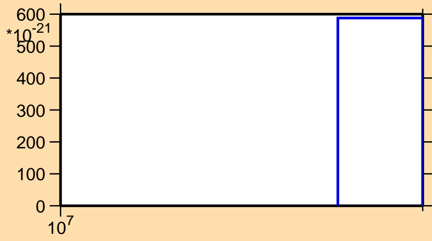
\sigma vs. E for ^{165}\text{Eu} (mt 42)
