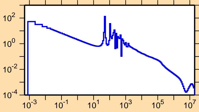
\sigma vs. E for ^{165}\text{Eu}(n,\gamma)
