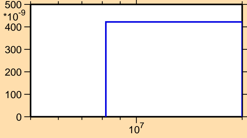
\sigma vs. E for ^{165}\text{Eu}(n,n\alpha)
