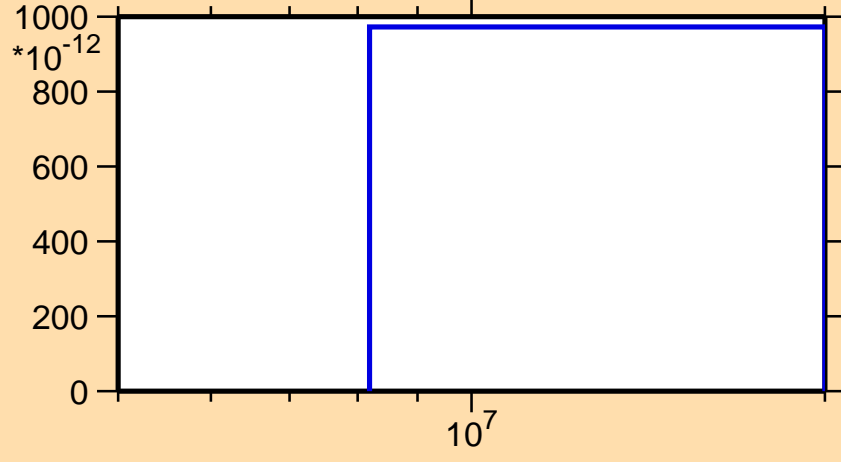
\sigma vs. E for ^{165}\text{Eu}(n,nd)
