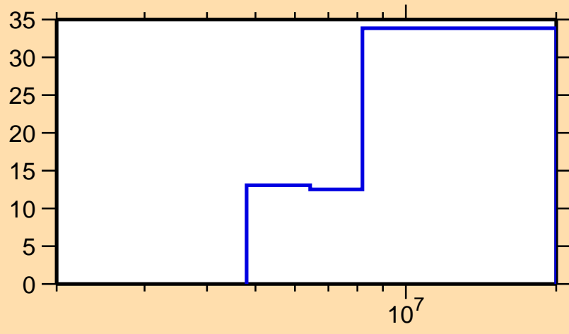
\Delta\sigma/\sigma vs. E for ^{165}\text{Eu}(n,2n)
