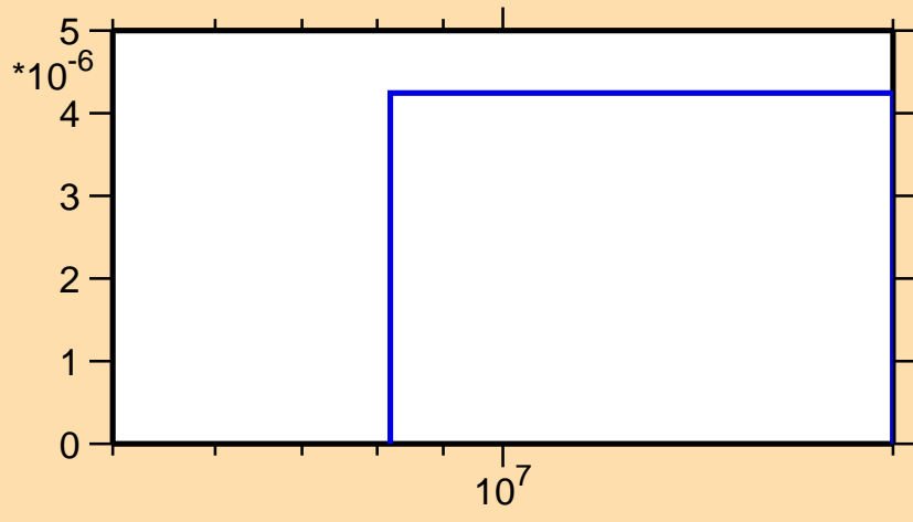
\sigma vs. E for ^{165}\text{Eu}(n,t)
