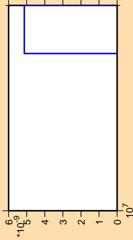
\Delta\sigma/\sigma vs. E for ^{166}\text{Eu} (mt 42)
