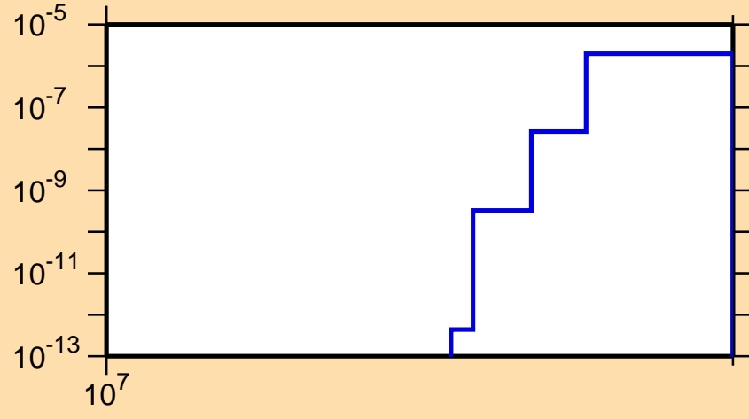
\sigma vs. E for ^{166}\text{Eu}(n,nd)
