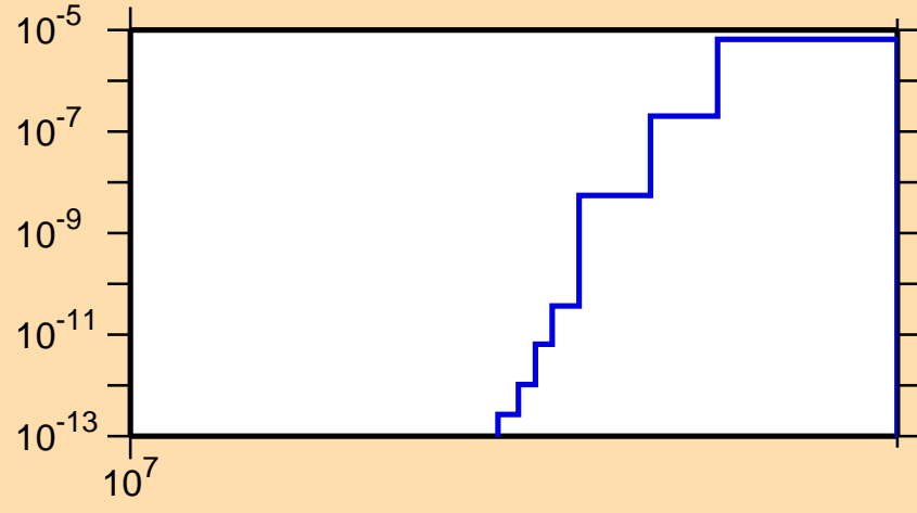
\sigma vs. E for ^{166}\text{Eu}(n,nt)
