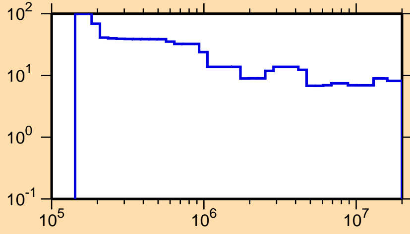
\Delta\sigma/\sigma vs. E for ^{166}\text{Eu}(n,\text{nonel.})
