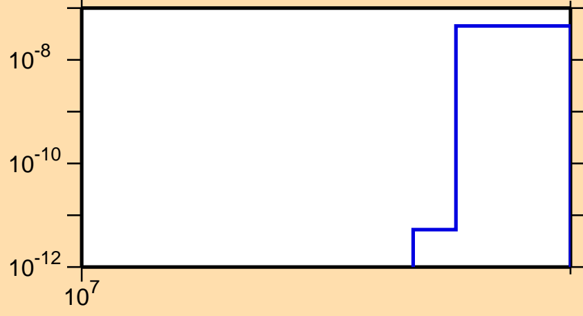
\sigma vs. E for ^{166}\text{Eu}(n,2np)
