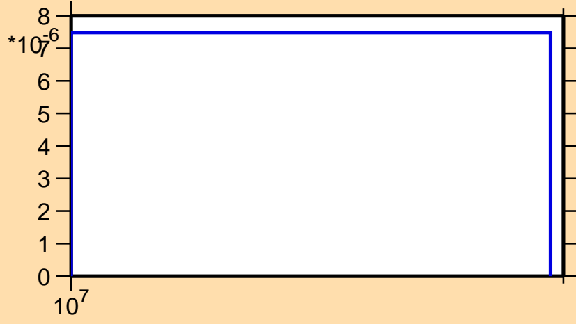
\sigma vs. E for ^{166}\text{Eu}(n,d)
