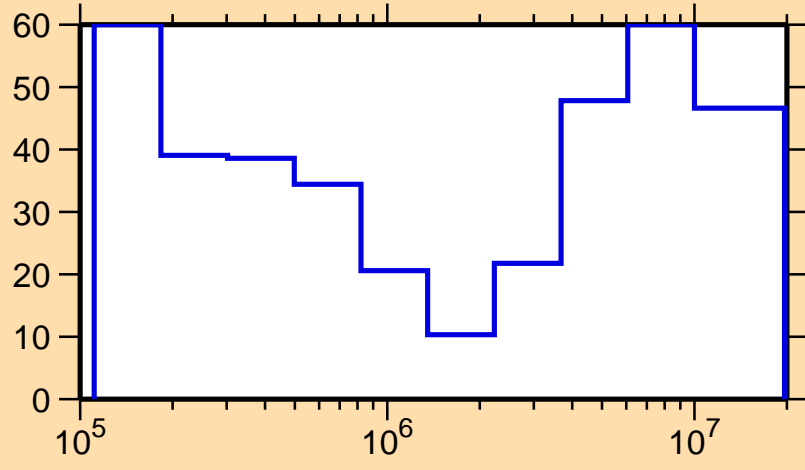
\Delta\sigma/\sigma vs. E for ^{166}\text{Eu}(n,\text{inel.})
