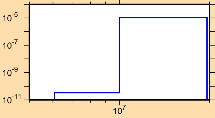
\sigma vs. E for ^{166}\text{Eu}(n,\alpha)
