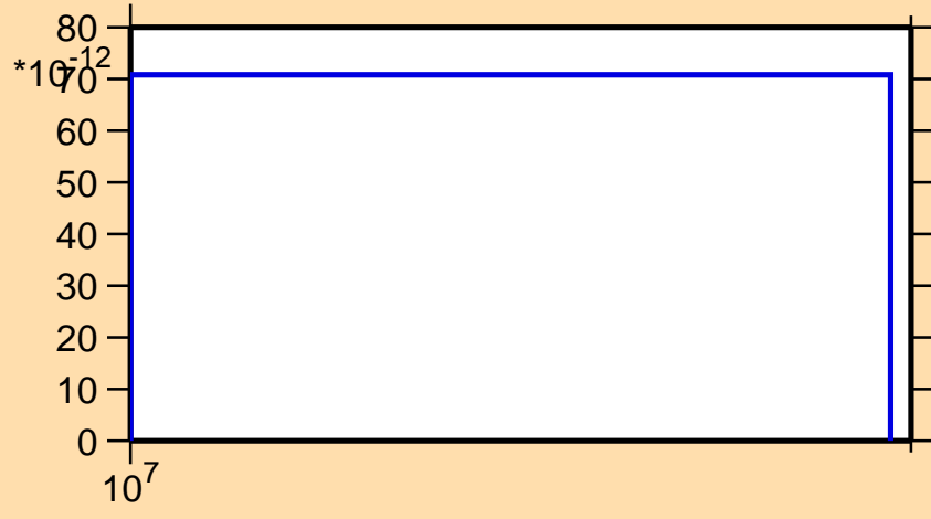
\sigma vs. E for ^{166}\text{Eu}(n,2n\alpha)
