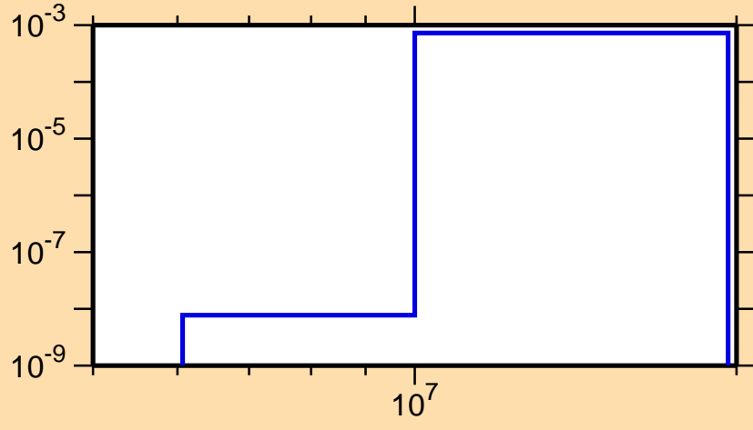
\sigma vs. E for ^{166}\text{Eu}(n,p)
