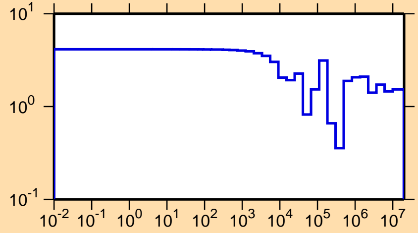
\Delta\sigma/\sigma vs. E for ^{17}\text{F}(n,\text{el.})
