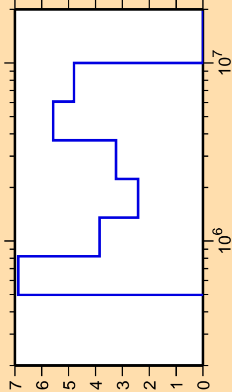
\Delta\sigma/\sigma vs. E for ^{17}\text{F}(n,n_1)
