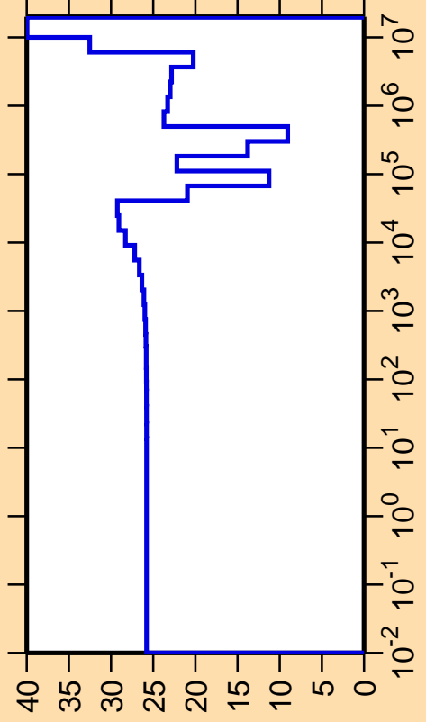
\Delta\sigma/\sigma vs. E for ^{17}\text{F}(n,\gamma)
