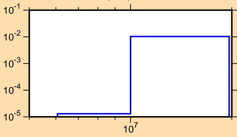
\sigma vs. E for ^{21}\text{F}(n,\alpha)
