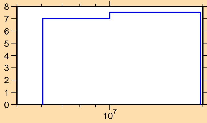
\Delta\sigma/\sigma vs. E for ^{21}\text{F}(n,ncont.)
