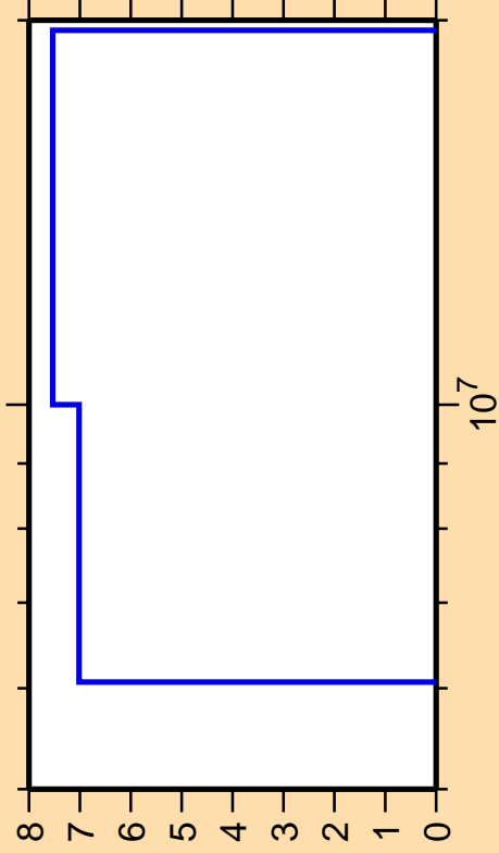
\Delta\sigma/\sigma vs. E for ^{21}\text{F}(n,n\text{cont.})
