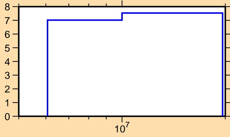
\Delta\sigma/\sigma vs. E for ^{21}\text{F}(n,n\text{cont.})
