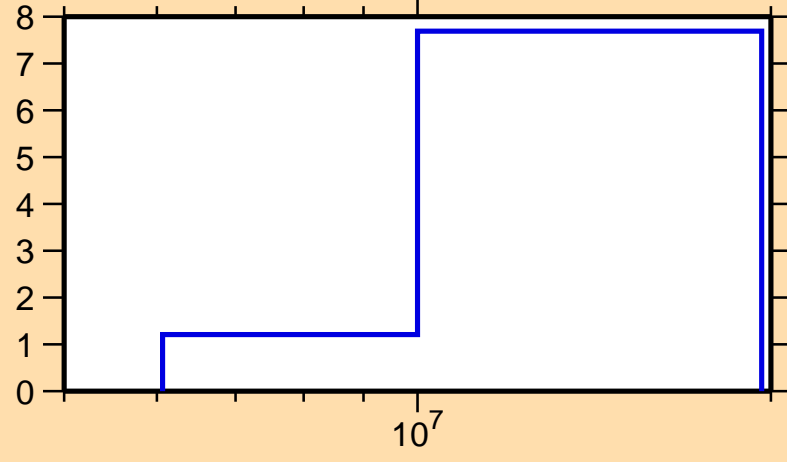
\Delta\sigma/\sigma vs. E for ^{21}\text{F}(n,n_1)
