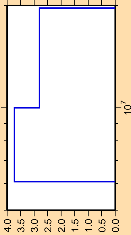
\Delta\sigma/\sigma vs. E for ^{21}\text{F}(n,2n)
