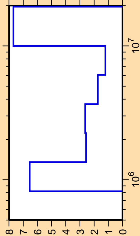
\Delta\sigma/\sigma vs. E for ^{21}\text{F}(n,n_1)
