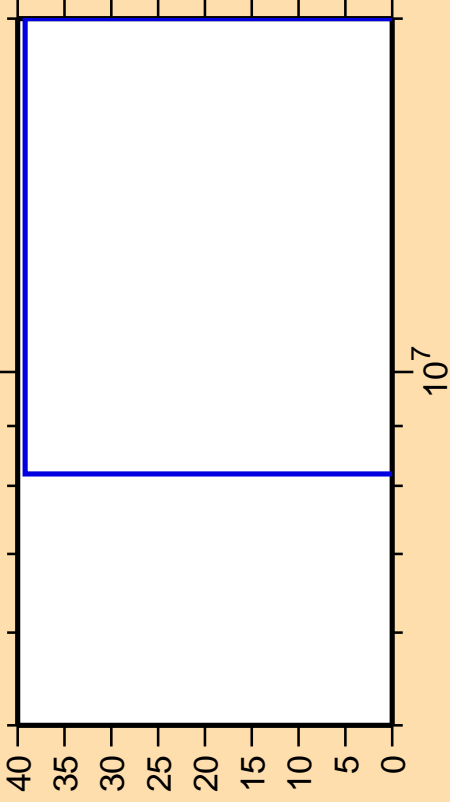
\Delta\sigma/\sigma vs. E for ^{21}\text{F}(n,\gamma)
