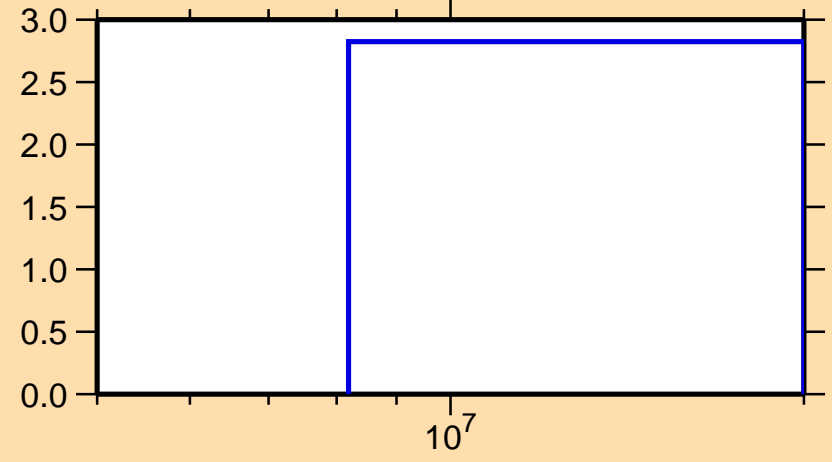
\Delta\sigma/\sigma vs. E for ^{21}\text{F}(n,2n)
