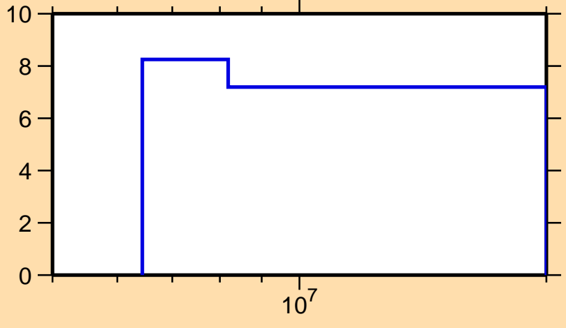
\Delta\sigma/\sigma vs. E for ^{21}\text{F}(n,n\text{cont.})
