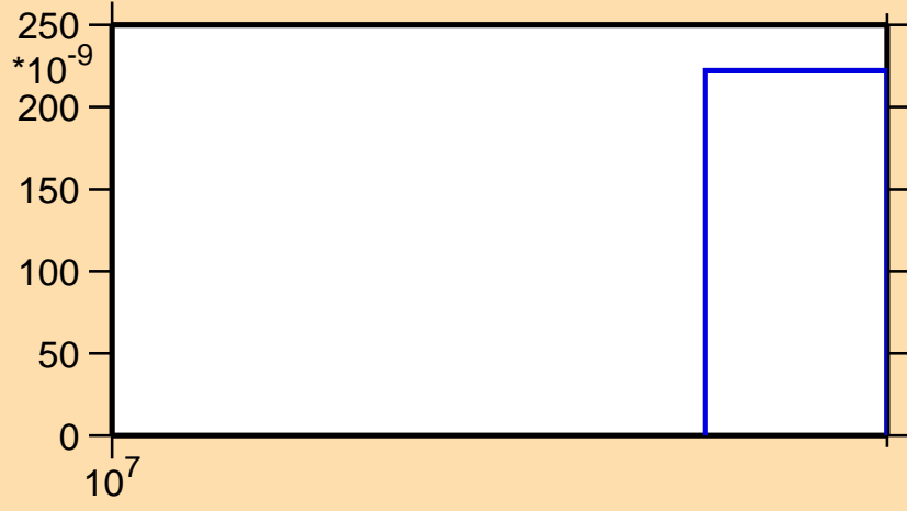
\sigma vs. E for ^{22}\text{F}(n,2np)
