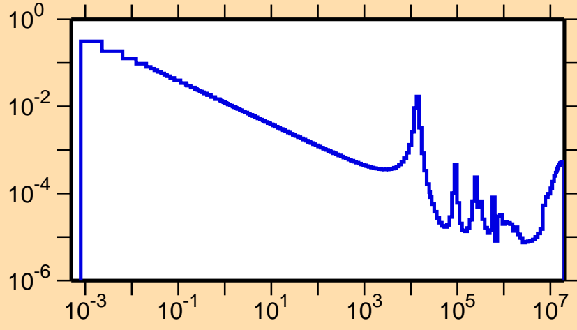
\sigma vs. E for ^{22}\text{F}(n,\gamma)
