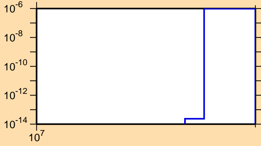
\sigma vs. E for ^{22}\text{F}(n,2n\alpha)
