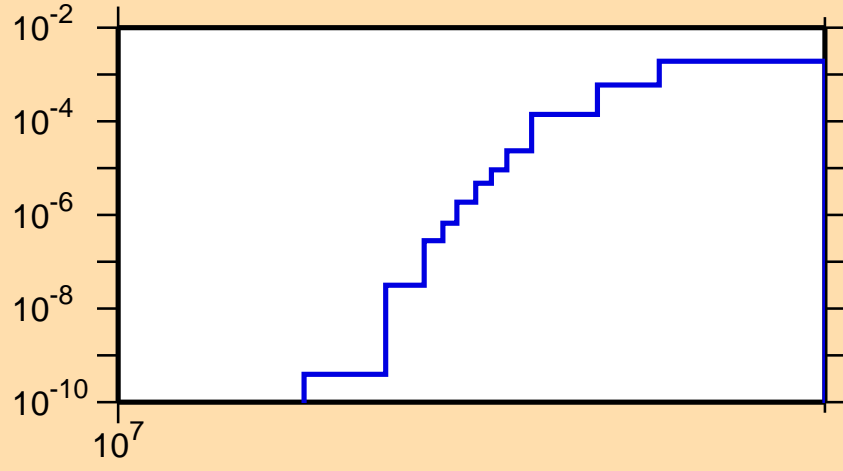
\sigma vs. E for ^{52}\text{Fe}(n,pd)
