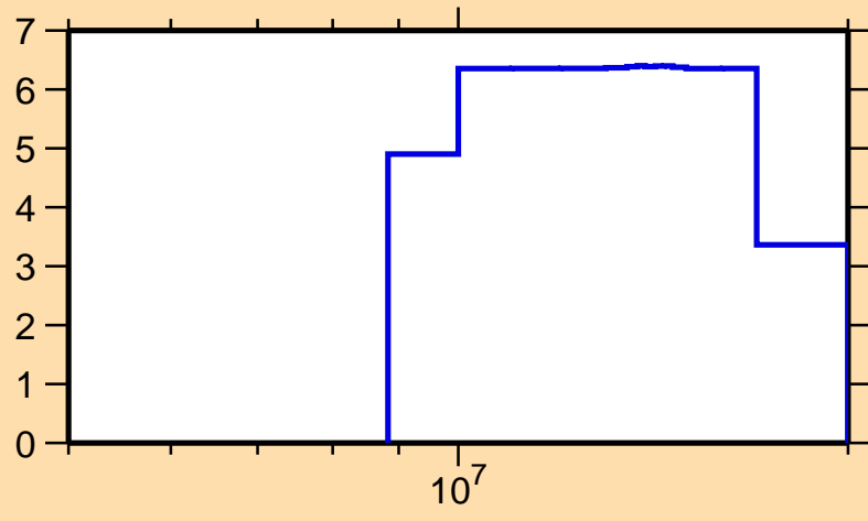
\Delta\sigma/\sigma vs. E for ^{52}\text{Fe}(n,\text{el.})
