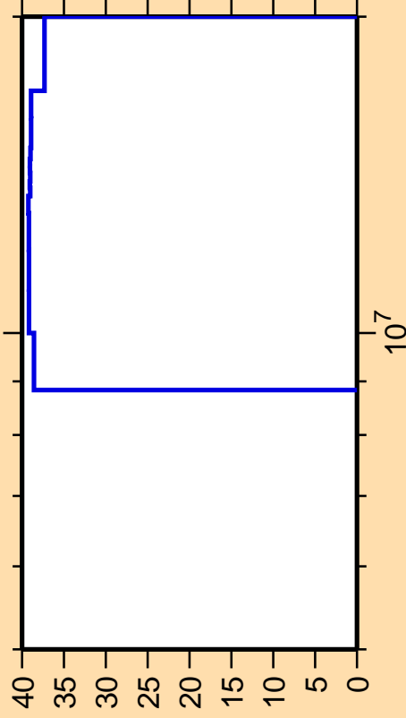
\Delta\sigma/\sigma vs. E for ^{52}\text{Fe}(n,n\text{cont.})
