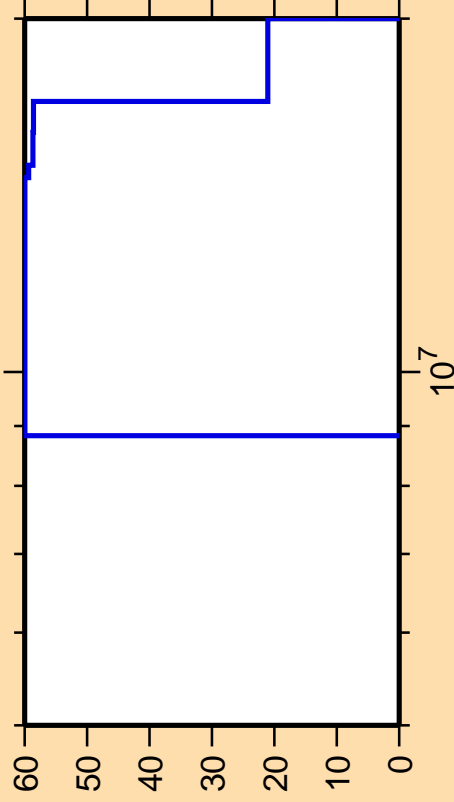
\Delta\sigma/\sigma vs. E for ^{52}\text{Fe}(n,2n)
