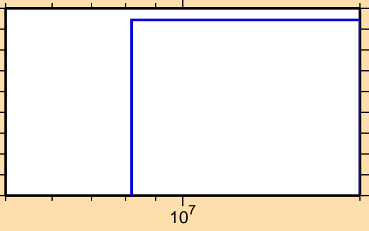
\sigma vs. E for ^{52}\text{Fe}(\text{mt117})
