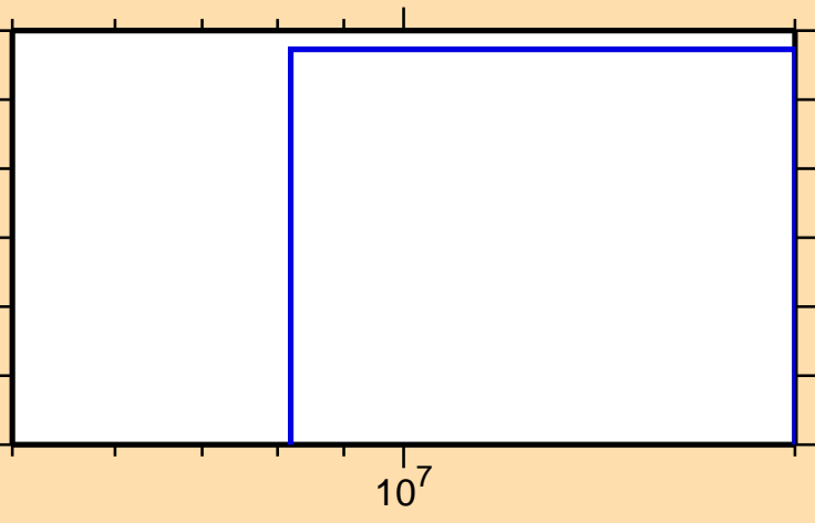
\sigma vs. E for ^{53}\text{Fe}(n,t)
