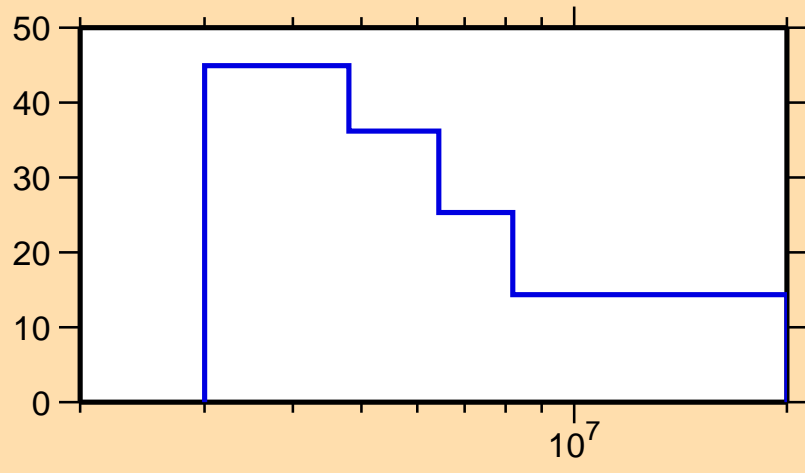
\Delta\sigma/\sigma vs. E for ^{53}\text{Fe}(n,ncont.)
