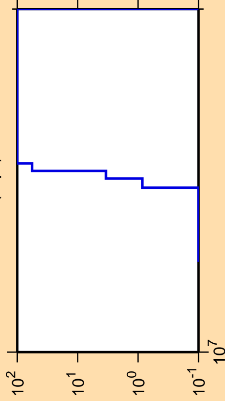
\Delta\sigma/\sigma vs. E for ^{53}\text{Fe}(n,pt)
