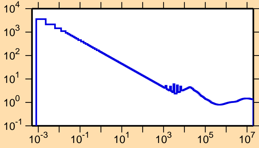
\sigma vs. E for ^{53}\text{Fe}(n,\text{nonel.})
