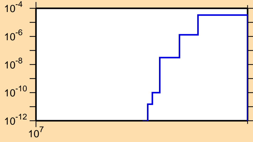
\sigma vs. E for ^{53}\text{Fe}(n,pt)
