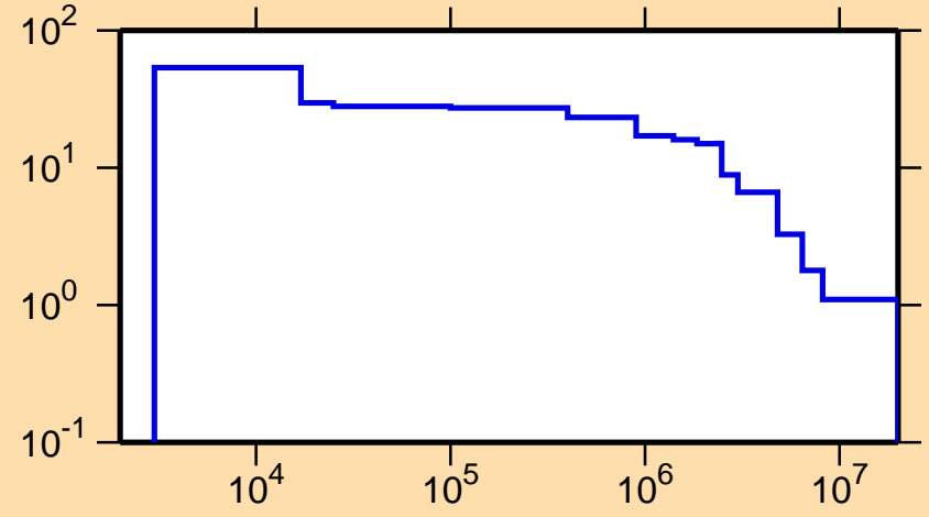
\Delta\sigma/\sigma vs. E for ^{53}\text{Fe}(n,\text{nonel.})
