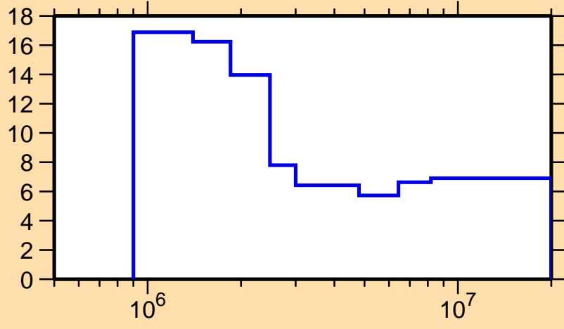
\Delta\sigma/\sigma vs. E for ^{54}\text{Fe}(n,p)
