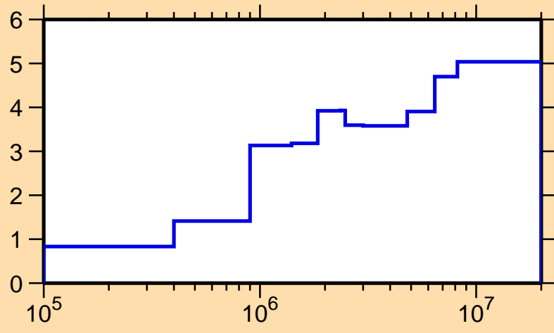
\Delta\sigma/\sigma vs. E for ^{54}\text{Fe}(n,el.)
