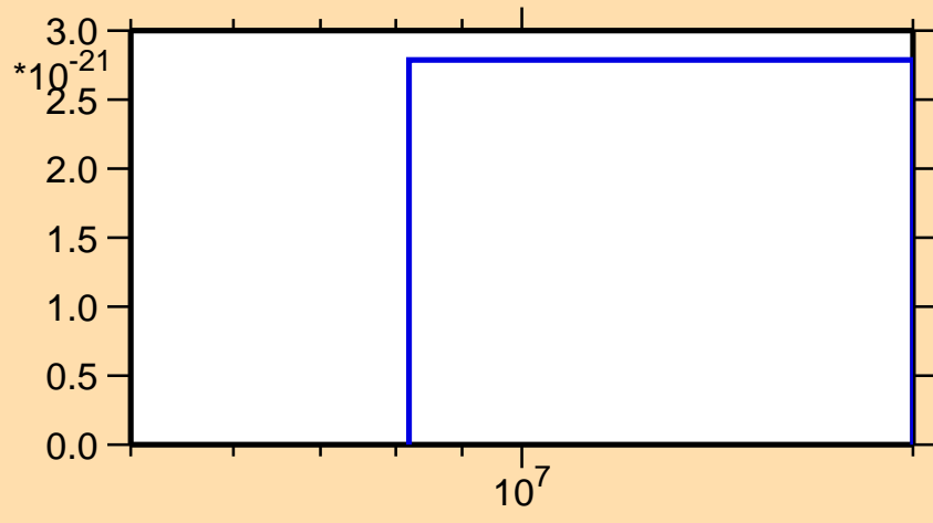
\sigma vs. E for ^{54}\text{Fe}(n,\text{pt})
