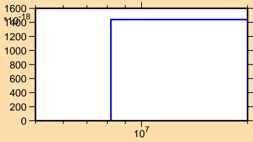
\sigma vs. E for ^{54}\text{Fe}(n,\text{nd})
