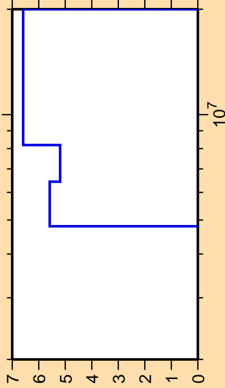
\Delta\sigma/\sigma vs. E for ^{54}\text{Fe}(n,\text{ncont.})
