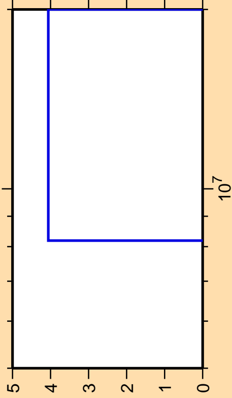
\Delta\sigma/\sigma vs. E for ^{54}\text{Fe}(n,np)
