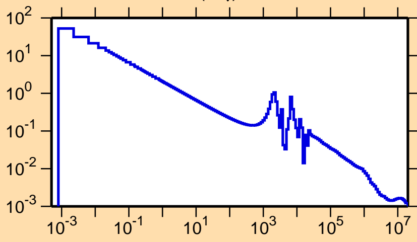
\sigma vs. E for ^{55}\text{Fe}(n,\gamma)
