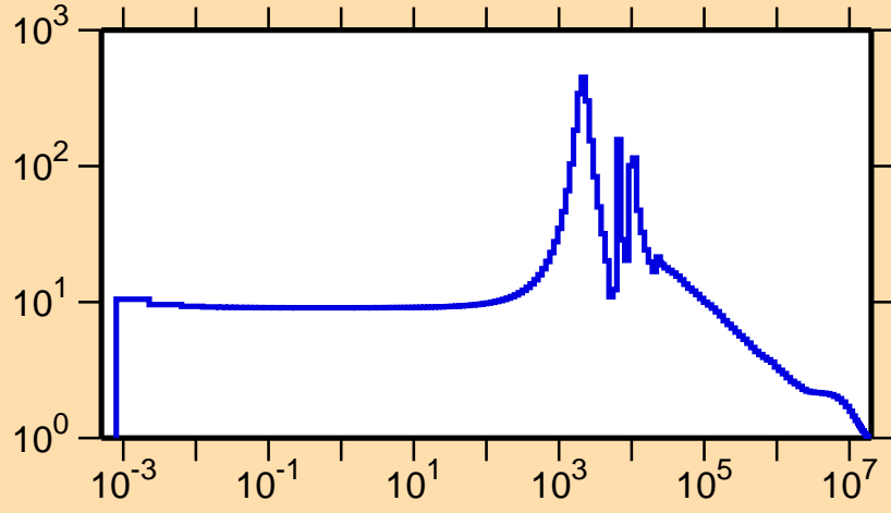
\sigma vs. E for ^{55}\text{Fe}(n,\text{el.})
