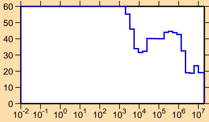
\Delta\sigma/\sigma vs. E for ^{55}\text{Fe}(n,p)
