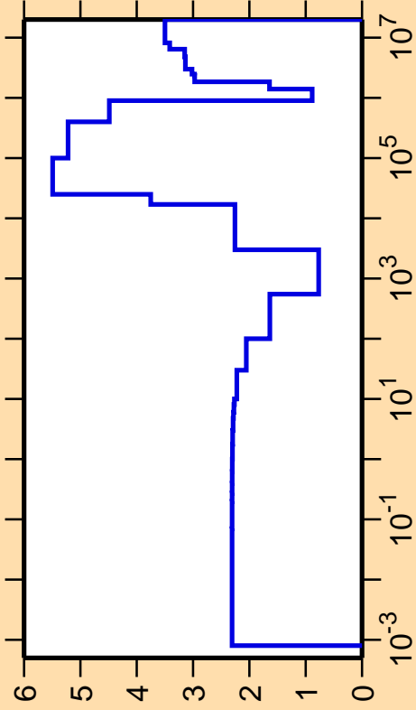
\Delta\sigma/\sigma vs. E for ^{55}\text{Fe}(n,\text{el.})
