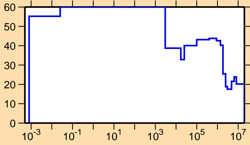
\Delta\sigma/\sigma vs. E for ^{55}\text{Fe}(n,p)
