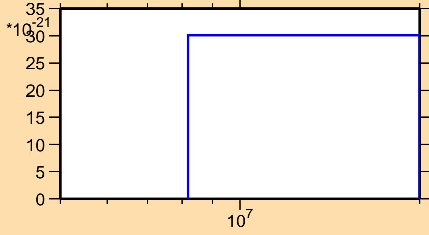
\sigma vs. E for ^{55}\text{Fe}(n,2n\alpha)
