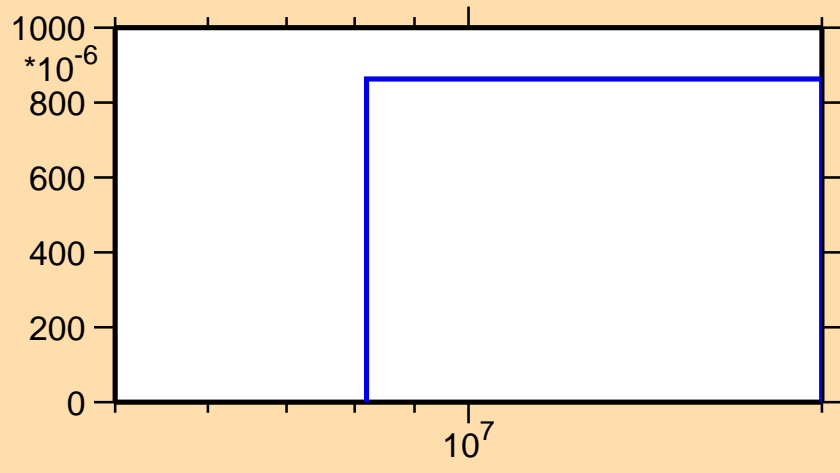
\sigma vs. E for ^{55}\text{Fe}(n,\alpha)
