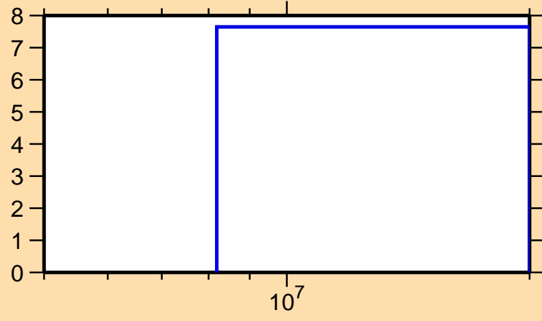
\Delta\sigma/\sigma vs. E for ^{55}\text{Fe}(n,\text{inel.})
