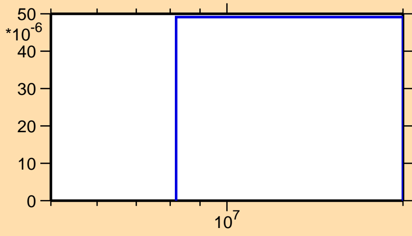
\sigma vs. E for ^{55}\text{Fe}(n,p\alpha)
