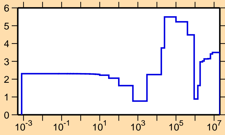
\Delta\sigma/\sigma vs. E for ^{55}\text{Fe}(n,\text{el.})
