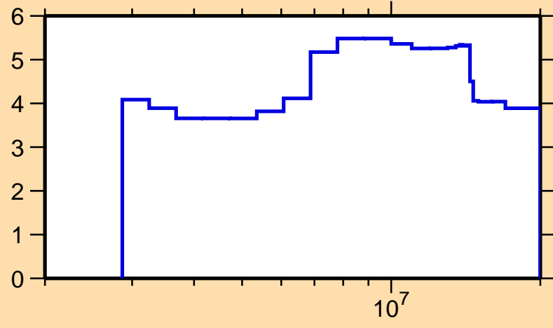
\Delta\sigma/\sigma vs. E for ^{56}\text{Fe}(n,el.)
