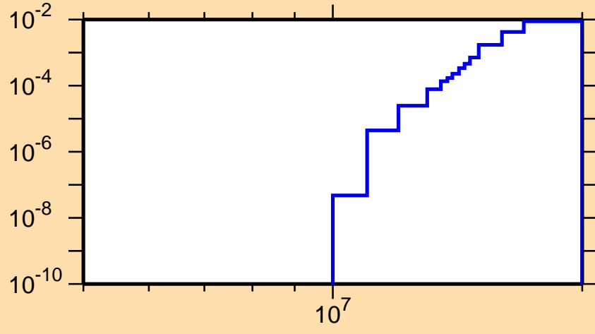
\sigma vs. E for ^{56}\text{Fe}(n,n\alpha)
