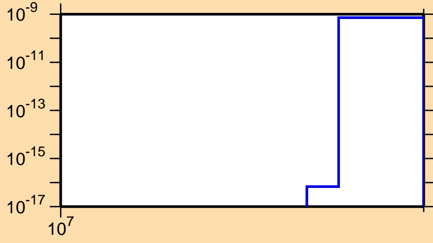
\sigma vs. E for ^{56}\text{Fe}(n,pd)
