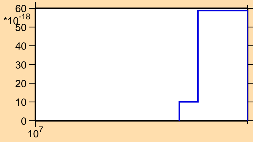
\sigma vs. E for ^{56}\text{Fe}(\text{mt117})
