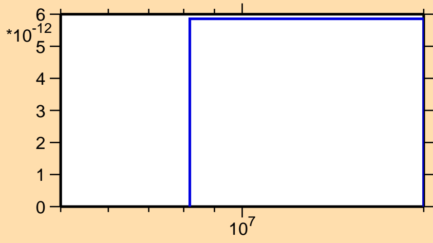
\sigma vs. E for ^{56}\text{Fe}(n,\text{pd})
