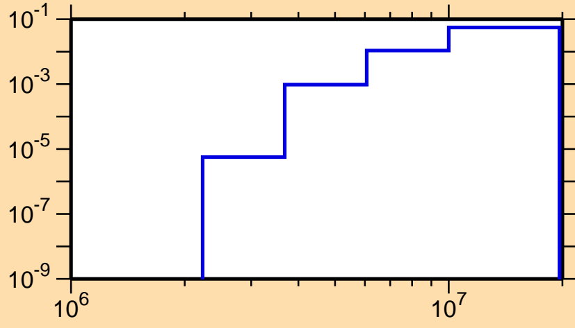
\sigma vs. E for ^{57}\text{Fe}(n,p)
