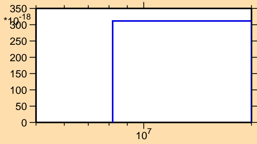
\sigma vs. E for ^{60}\text{Fe}(n,\text{nd})
