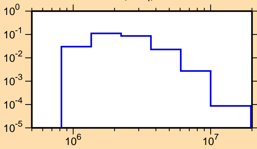
\sigma vs. E for ^{61}\text{Fe}(n,n_4)
