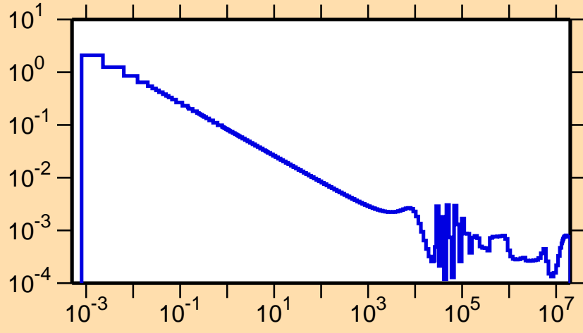
\sigma vs. E for ^{62}\text{Fe}(n,\gamma)
