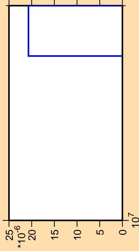
\Delta\sigma/\sigma vs. E for ^{62}\text{Fe}(n,nd)
