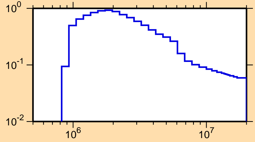
\sigma vs. E for ^{62}\text{Fe}(n,n_1)
