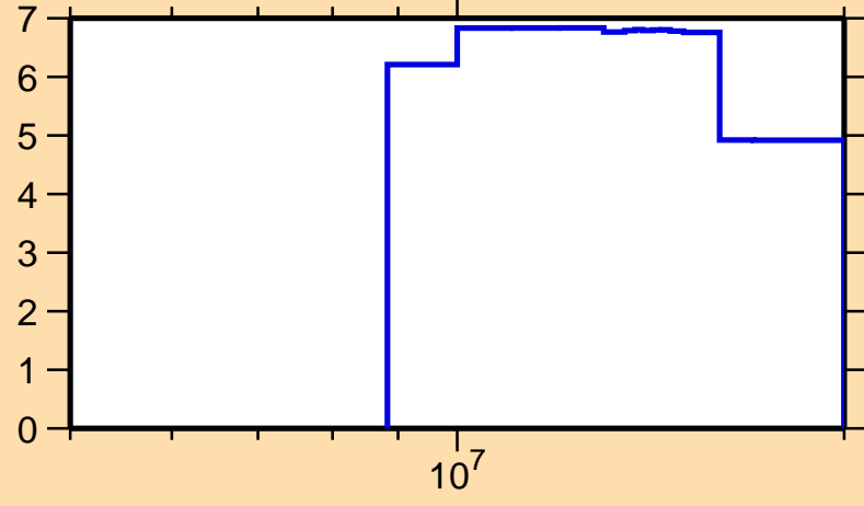
\Delta\sigma/\sigma vs. E for ^{62}\text{Fe}(n,el.)
