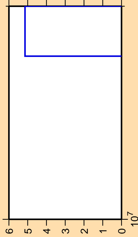
\Delta\sigma/\sigma vs. E for ^{62}\text{Fe}(n,nt)
