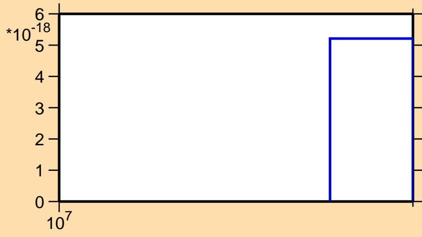
\sigma vs. E for ^{62}\text{Fe}(n,nd)
