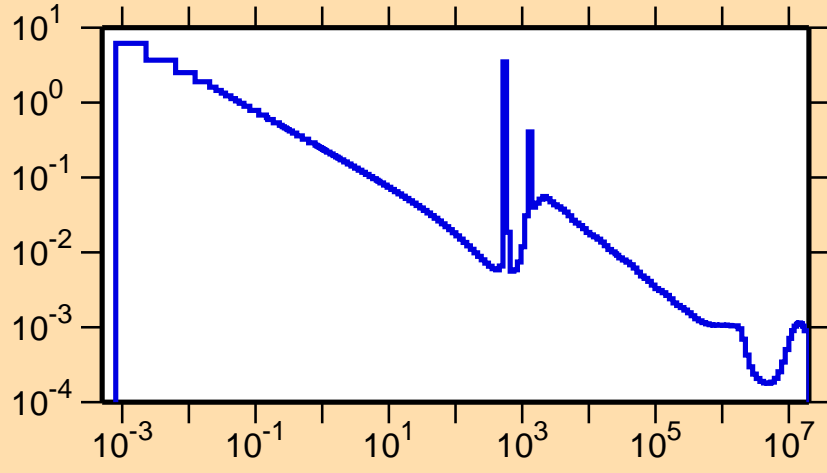
\sigma vs. E for ^{63}\text{Fe}(n,\gamma)
