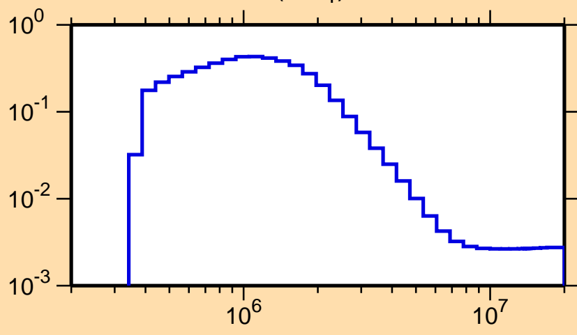
\sigma vs. E for ^{63}\text{Fe}(n,n_1)
