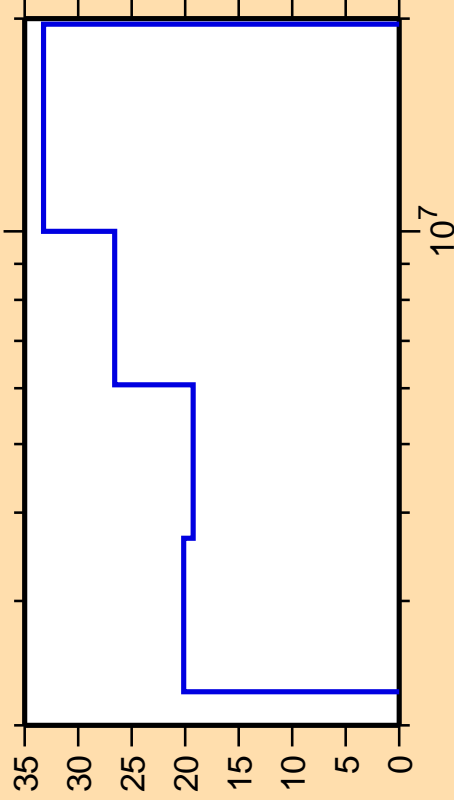
\Delta\sigma/\sigma vs. E for ^{63}\text{Fe}(n,n_{\text{cont}})
