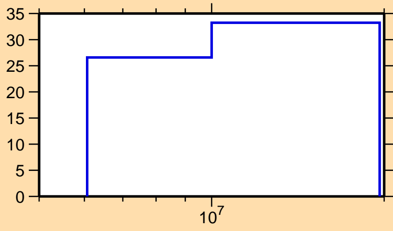
\Delta\sigma/\sigma vs. E for ^{63}\text{Fe}(n,ncont.)
