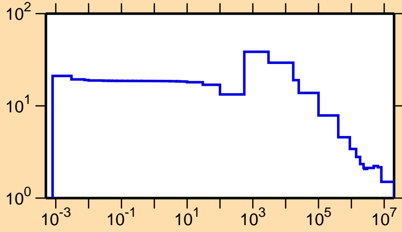
\sigma vs. E for ^{63}\text{Fe}(n,\text{el.})
