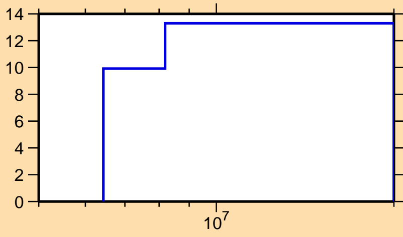
\Delta\sigma/\sigma vs. E for ^{63}\text{Fe}(n,el.)
