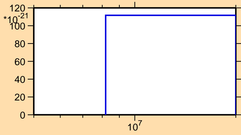
\sigma vs. E for ^{63}\text{Fe}(n,2np)
