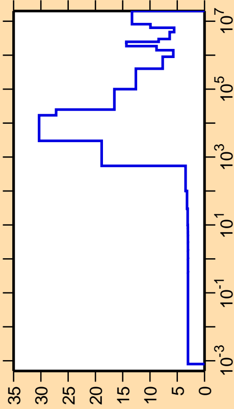
\Delta\sigma/\sigma vs. E for ^{63}\text{Fe}(n,\text{el.})
