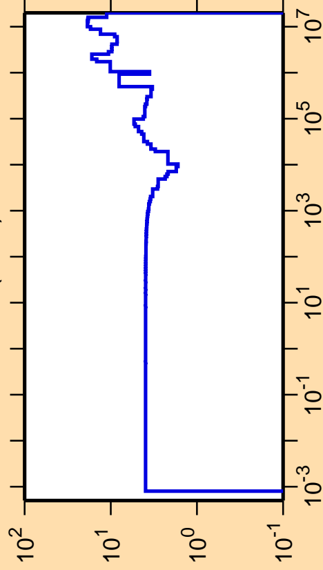
\Delta\sigma/\sigma vs. E for ^{64}\text{Fe}(n,\text{el.})
