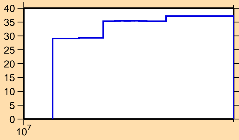
\Delta\sigma/\sigma vs. E for ^{64}\text{Fe}(n,ncont.)
