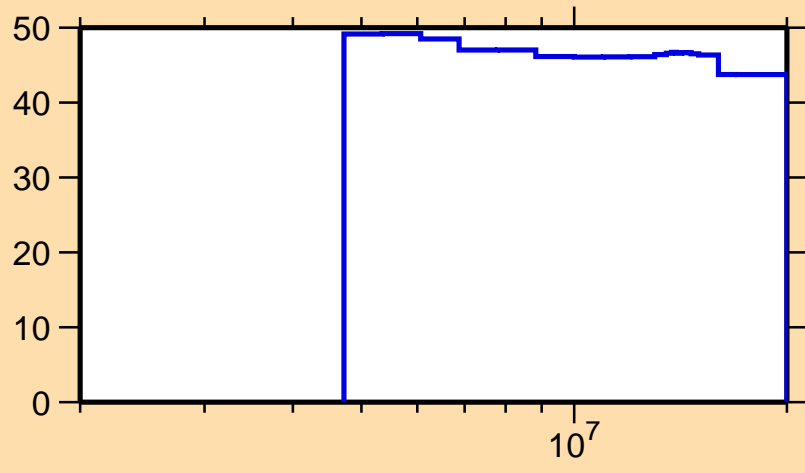
\Delta\sigma/\sigma vs. E for ^{64}\text{Fe}(n,n_1)
