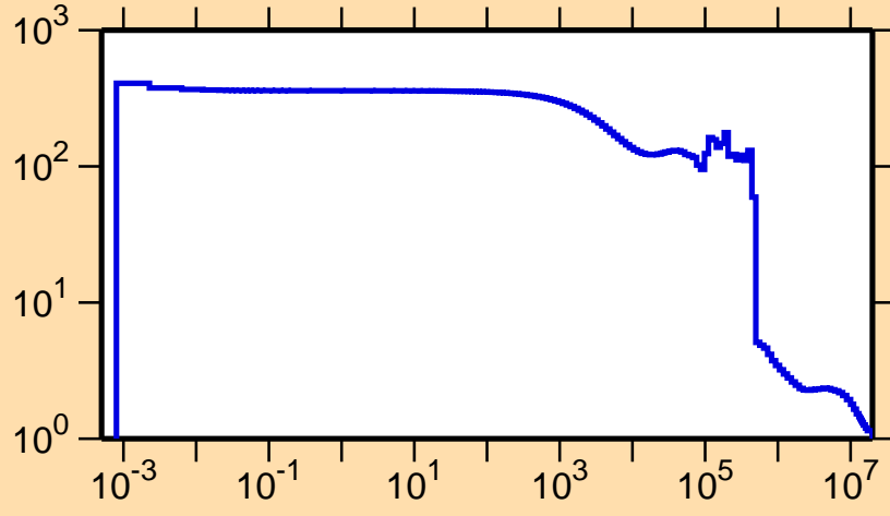
\sigma vs. E for ^{64}\text{Fe}(n,\text{el.})
