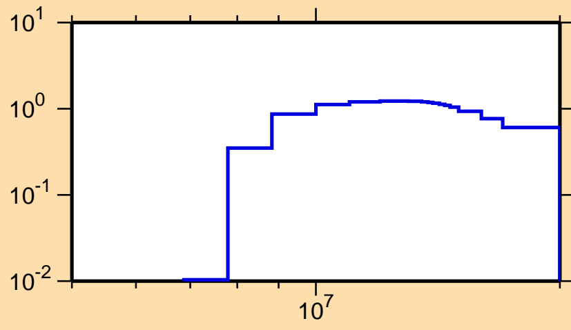
\sigma vs. E for ^{64}\text{Fe}(n,2n)
