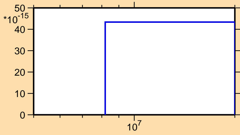
\sigma vs. E for ^{64}\text{Fe}(n,nt)
