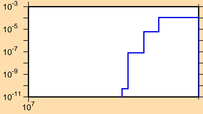
\sigma vs. E for ^{65}\text{Fe}(n,d)
