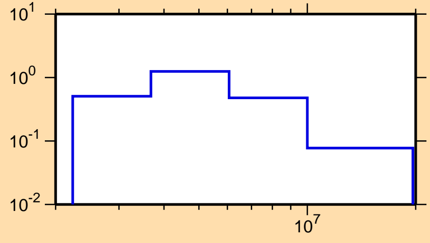
\sigma vs. E for ^{65}\text{Fe}(n,n\text{cont.})
