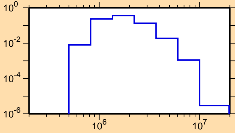
\sigma vs. E for ^{65}\text{Fe}(n,n_4)
