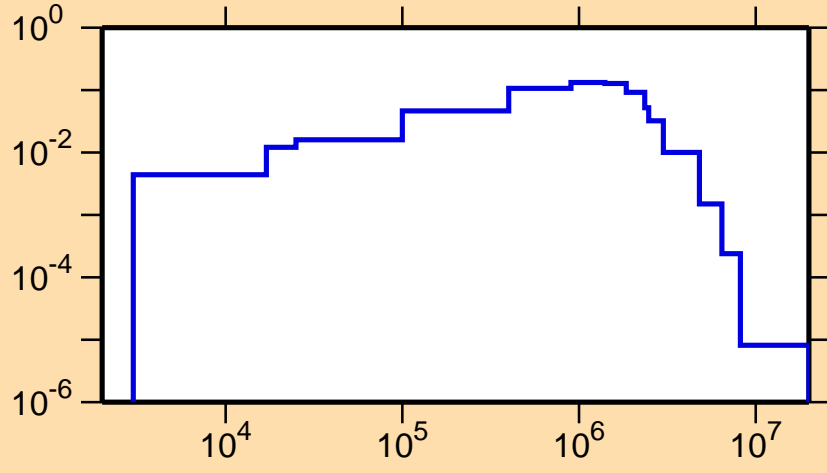
\sigma vs. E for ^{65}\text{Fe}(n,n_2)
