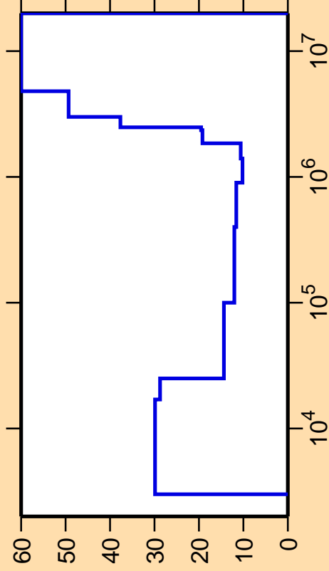
\Delta\sigma/\sigma vs. E for ^{65}\text{Fe}(n,n_2)
