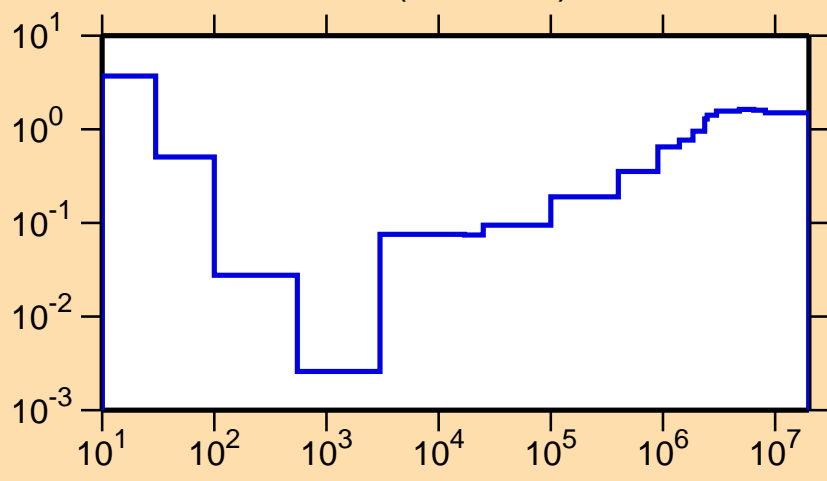
\sigma vs. E for ^{65}\text{Fe}(n,\text{nonel.})
