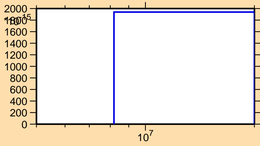
\sigma vs. E for ^{65}\text{Fe}(n,2n\alpha)
