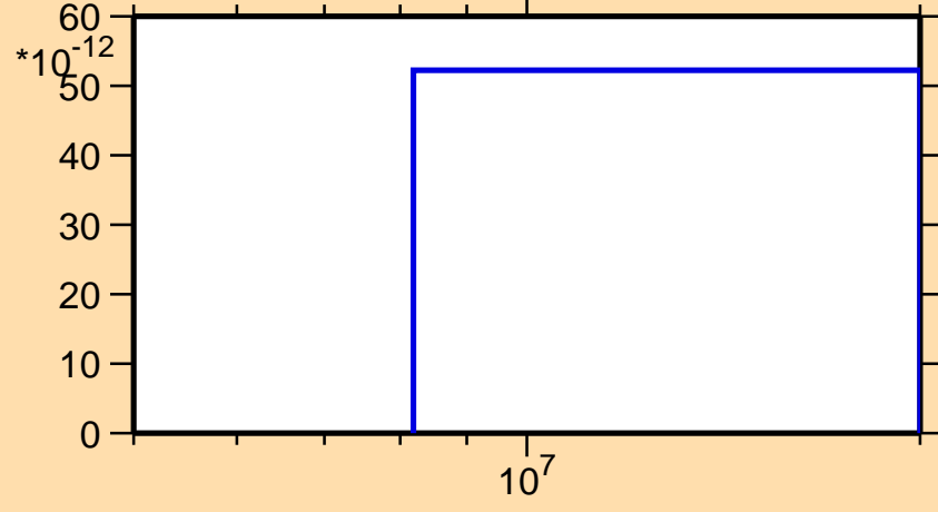
\sigma vs. E for ^{247}\text{Fm}(n,nd)
