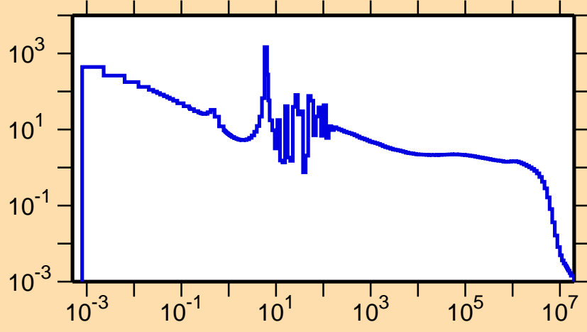
\sigma vs. E for ^{248}\text{Fm}(n,\gamma)
