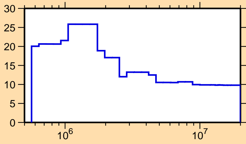
\Delta\sigma/\sigma vs. E for ^{248}\text{Fm}(n,nonel.)
