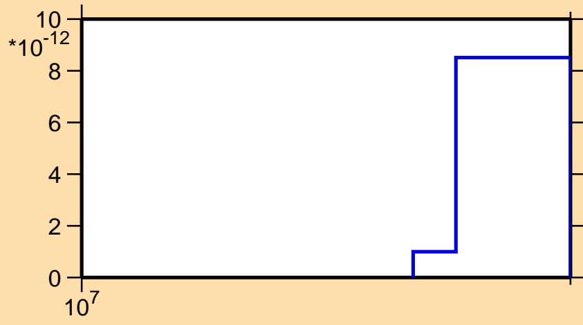
\sigma vs. E for ^{248}\text{Fm} (mt 45)
