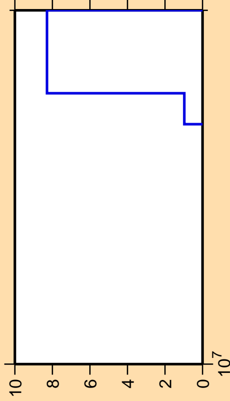
\Delta\sigma/\sigma vs. E for ^{248}\text{Fm} (mt 45)
