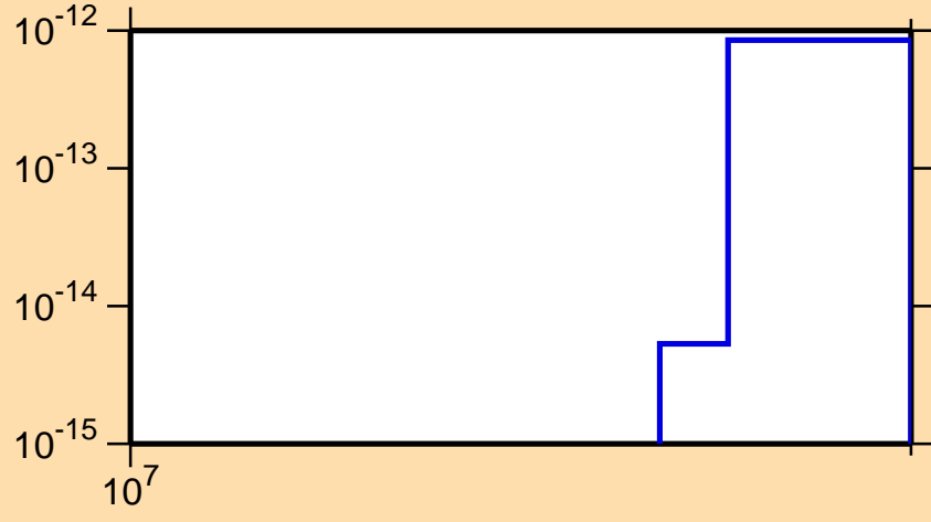
\sigma vs. E for ^{248}\text{Fm} (mt 34)
