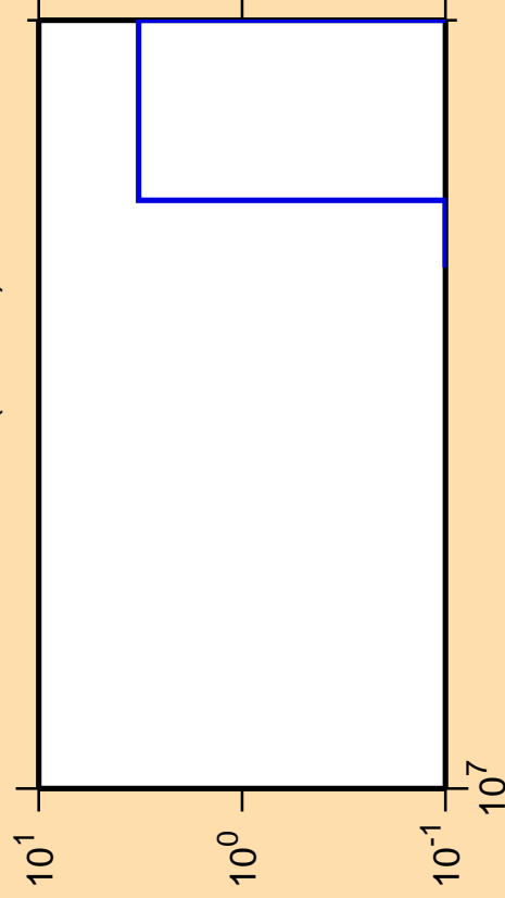
\Delta\sigma/\sigma vs. E for ^{248}\text{Fm} (mt 34)
