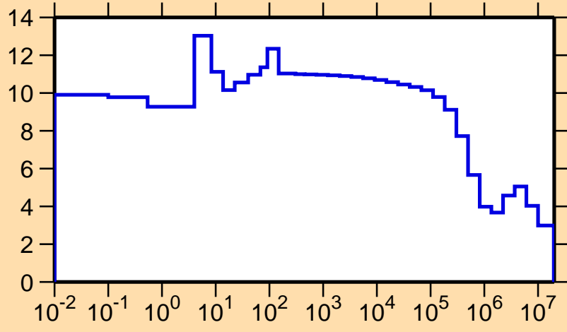
\sigma vs. E for ^{248}\text{Fm}(n,el.)
