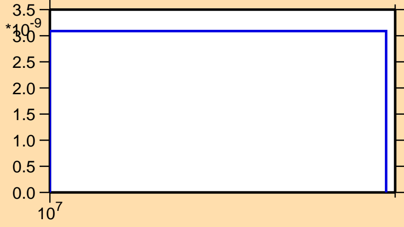
\sigma vs. E for ^{248}\text{Fm}(n,nt)
