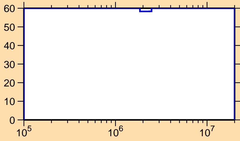
\Delta\sigma/\sigma vs. E for ^{248}\text{Fm}(n,\gamma)
