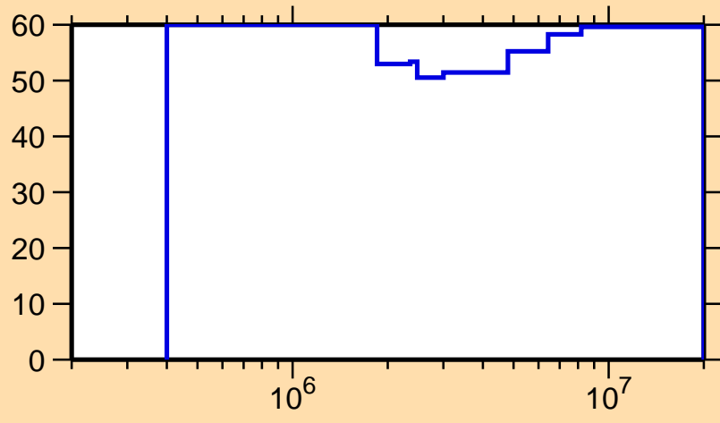
\Delta\sigma/\sigma vs. E for ^{248}\text{Fm}(n,n\text{cont.})
