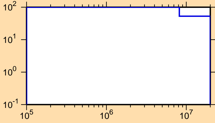
\Delta\sigma/\sigma vs. E for ^{248}\text{Fm}(n,p)
