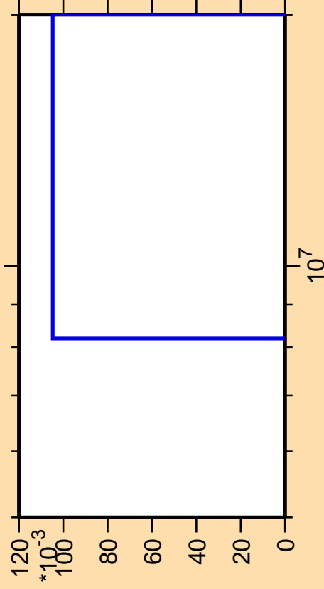
\Delta\sigma/\sigma vs. E for ^{248}\text{Fm} (mt 45)
