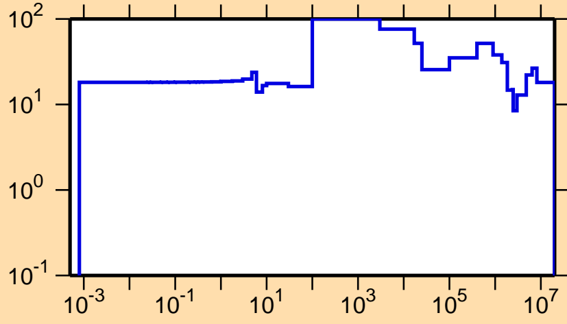
\Delta\sigma/\sigma vs. E for ^{248}\text{Fm}(n,el.)
