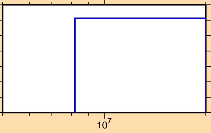
\sigma vs. E for ^{248}\text{Fm}(n,nd)
