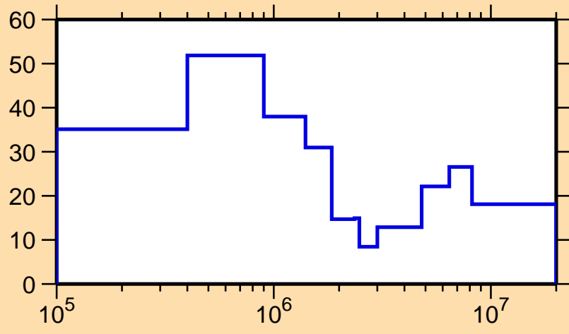
\Delta\sigma/\sigma vs. E for ^{248}\text{Fm}(n,el.)
