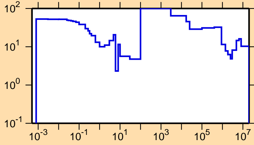
\Delta\sigma/\sigma vs. E for ^{248}\text{Fm}(n,tot.)
