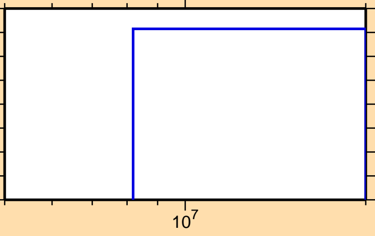
\sigma vs. E for ^{248}\text{Fm} (mt 34)
