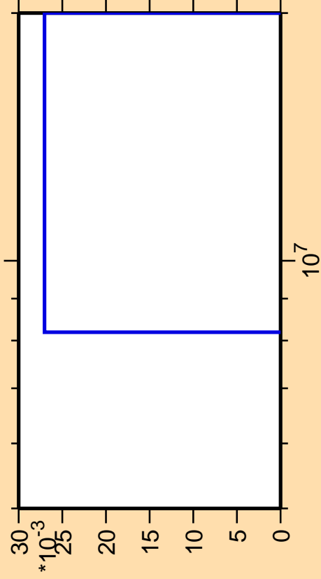
\Delta\sigma/\sigma vs. E for ^{248}\text{Fm} (mt 34)
