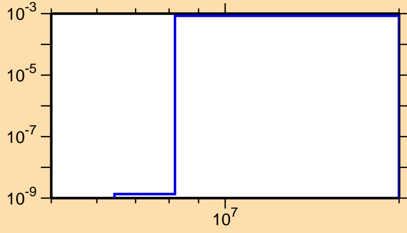
\sigma vs. E for ^{248}\text{Fm}(n,np)
