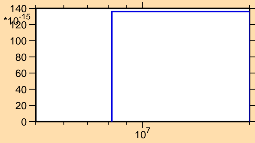
\sigma vs. E for ^{248}\text{Fm} (mt 45)
