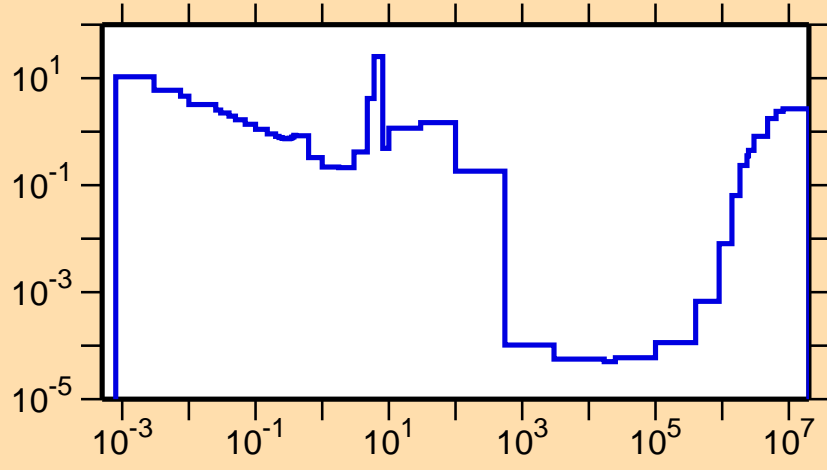
\sigma vs. E for ^{248}\text{Fm}(n,f)
