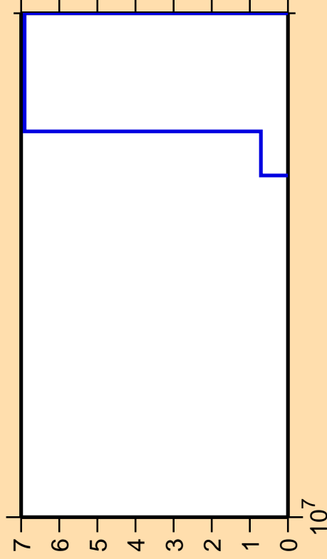
\Delta\sigma/\sigma vs. E for ^{250}\text{Fm} (mt 45)
