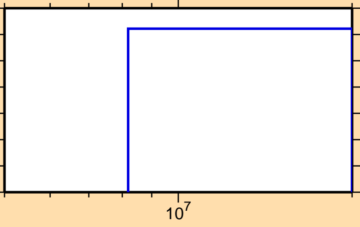
\sigma vs. E for ^{250}\text{Fm}(n,3n\alpha)
