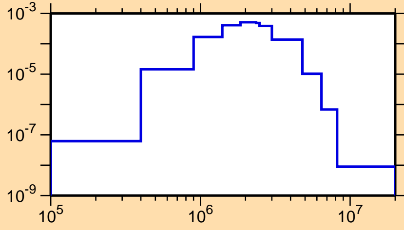
\sigma vs. E for ^{250}\text{Fm}(n,n_3)
