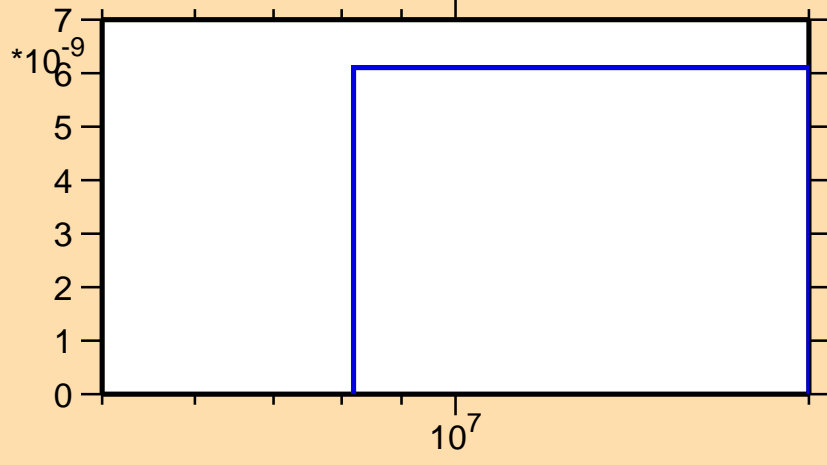
\sigma vs. E for ^{250}\text{Fm}(n,p\alpha)
