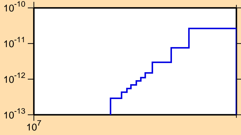
\sigma vs. E for ^{251}\text{Fm}(n,p\alpha)
