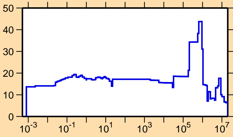
\Delta\sigma/\sigma vs. E for ^{251}\text{Fm}(n,el.)
