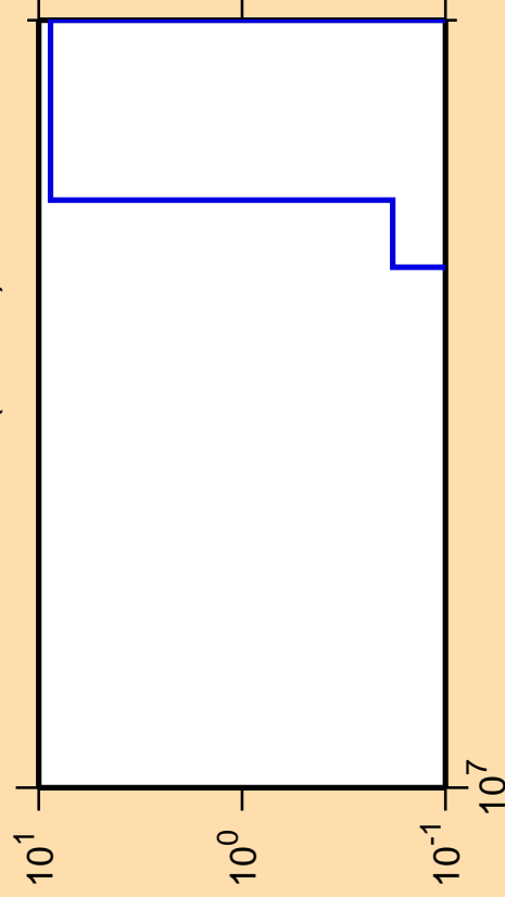
\Delta\sigma/\sigma vs. E for ^{251}\text{Fm} (mt 34)
