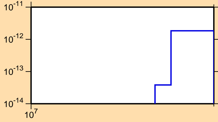
\sigma vs. E for ^{251}\text{Fm} (mt 34)
