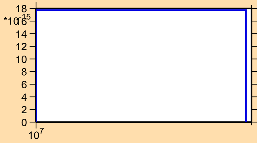
\sigma vs. E for ^{251}\text{Fm} (mt 34)
