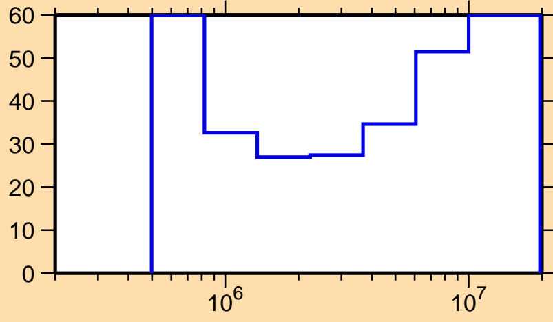
\Delta\sigma/\sigma vs. E for ^{251}\text{Fm}(n,n\text{cont.})
