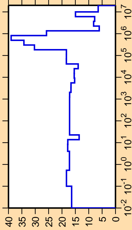
\Delta\sigma/\sigma vs. E for ^{251}\text{Fm}(n,\text{el.})
