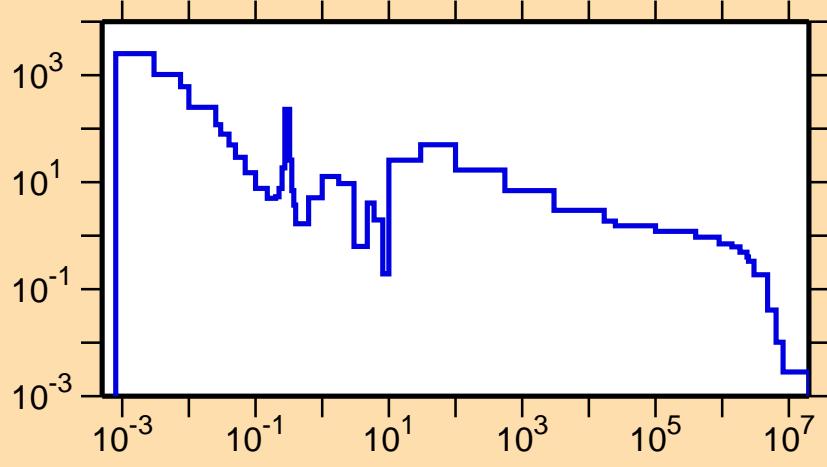
\sigma vs. E for ^{251}\text{Fm}(n,\gamma)
