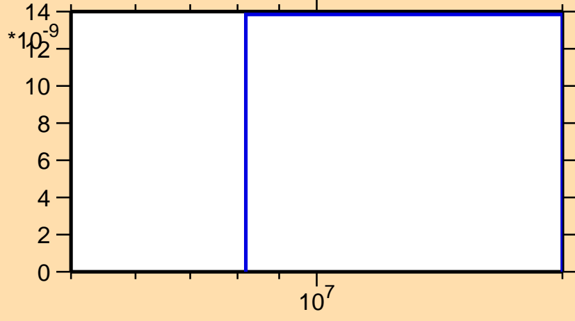
\sigma vs. E for ^{251}\text{Fm}(n,nd)
